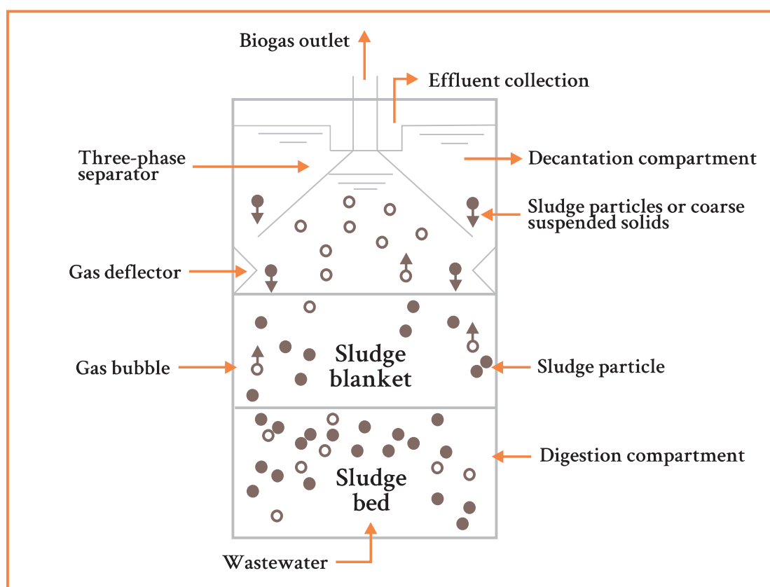
Figure 4. Operating scheme of a UASB biodigester.
