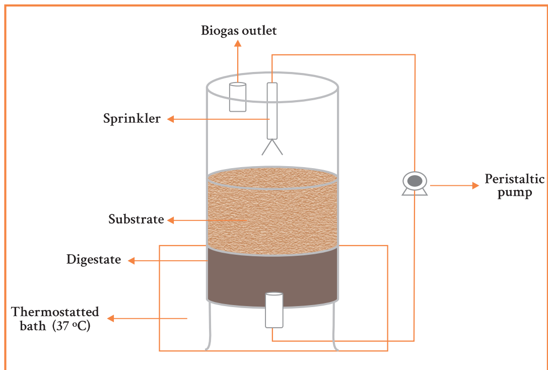
Figure 8. Solid-state batch biodigester with inoculum recirculation.
